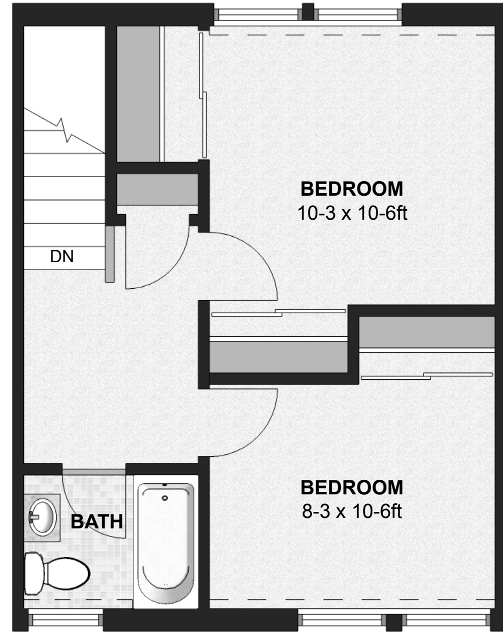
2nd FLOOR
